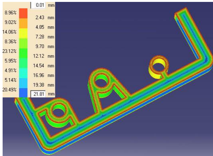
Figure 5(b): Rectified design
