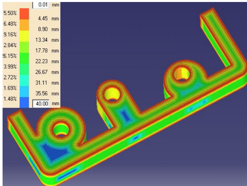
Figure 5(a): Design containing thick regions
