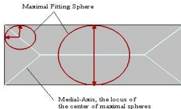
Figure 3: Sphere Method
