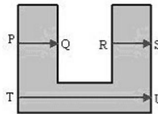
Figure 2: Ray Method
